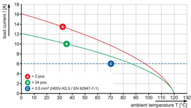
LSF-SMT 3.81/./90 3.5
