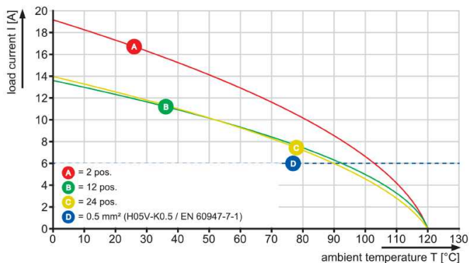
LSF-SMT 3.5/./180 3.5
