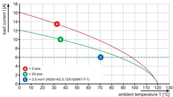
LSF-SMT 3.81/./90 3.5
