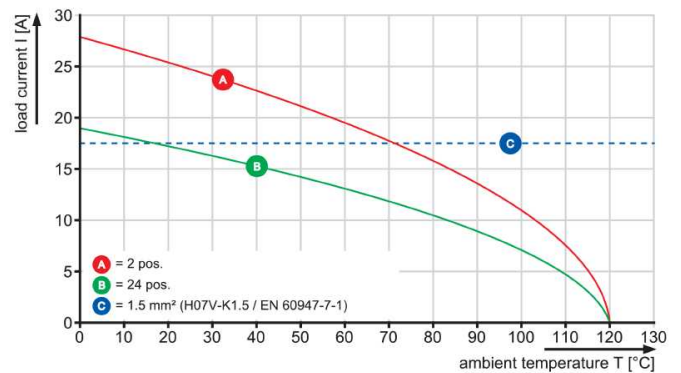
LSF-SMT 3.81/./90 3.5
