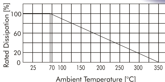
DERATING CURVE
