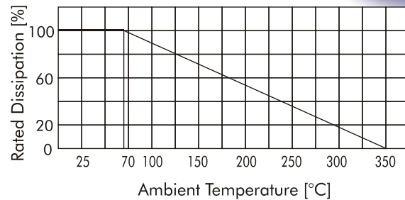
DERATING CURVE
