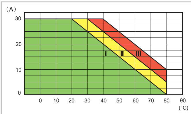
L77-4 Output RMS current vs. ambient temperature 77.31.x.xxx.80xx
