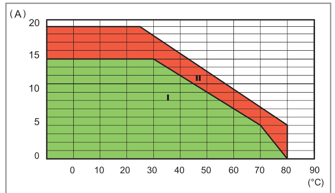
L77-6 Output RMS current vs. ambient temperature 77.11.x.xxx.82xx
