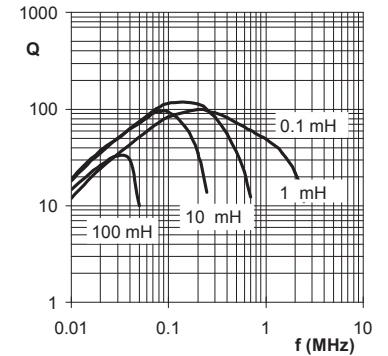
Typical Q vs Frequency(f)
