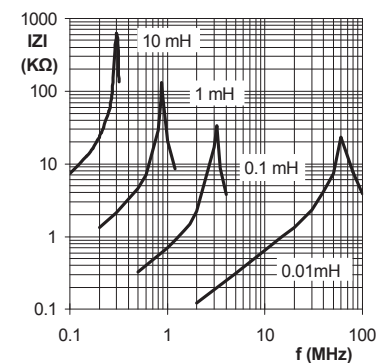
Typical IZI vs Frequency(f)
