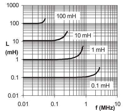
Typical L vs Frequency(f)
