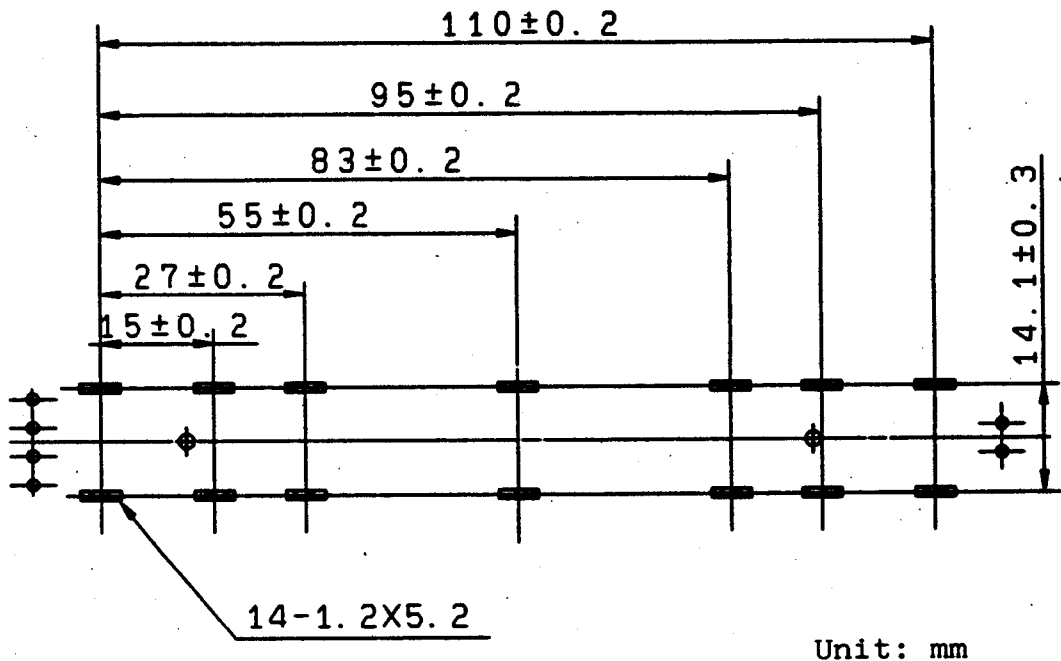
Viewed from mounting side 挿入側より
