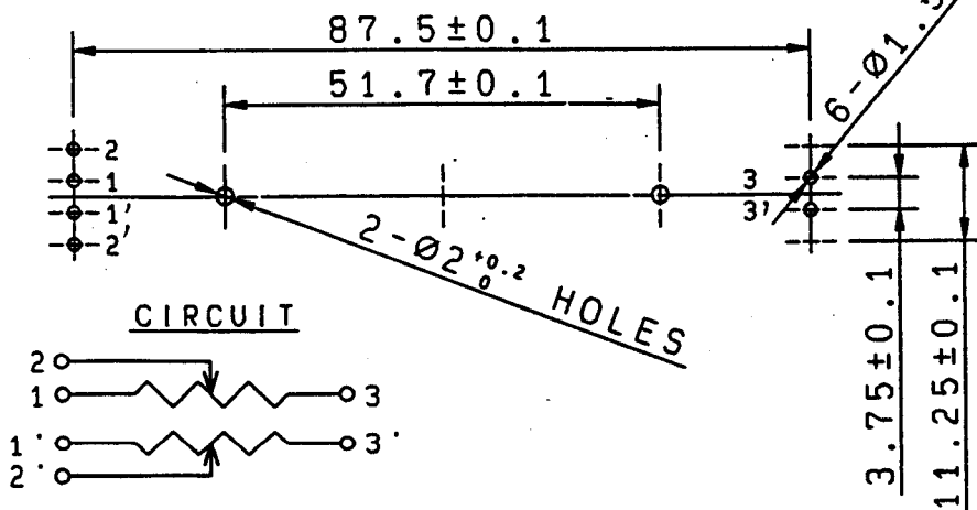
MOUNTING HOLE DETAIL (取付穴寸法図) VIEWED FROM MOUNTING SIDE (挿入側より)
