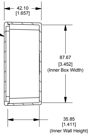
SECTION A-A End View of Assembly
