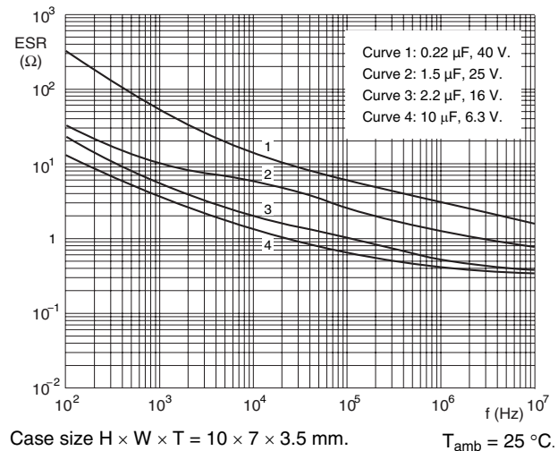
Fig.13 Typical ESR as a function of frequency.
