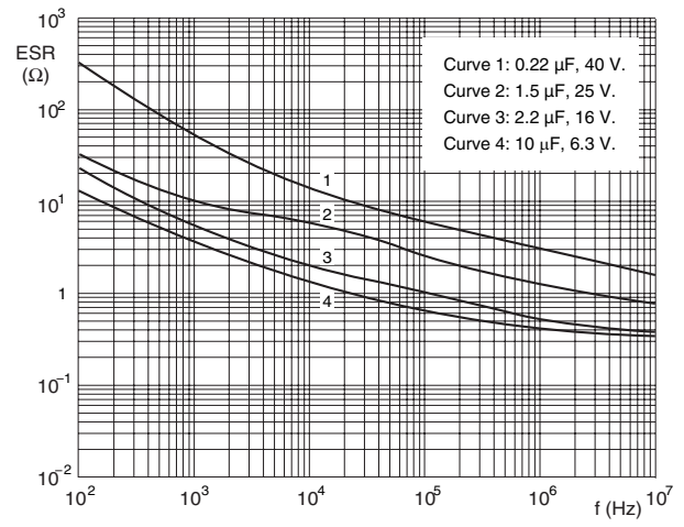
Case size H \times W \times T = 10 \times 7 \times 3.5 mm. T_{amb} = 25^\circ\text{C} . Fig.13 Typical ESR as a function of frequency.
