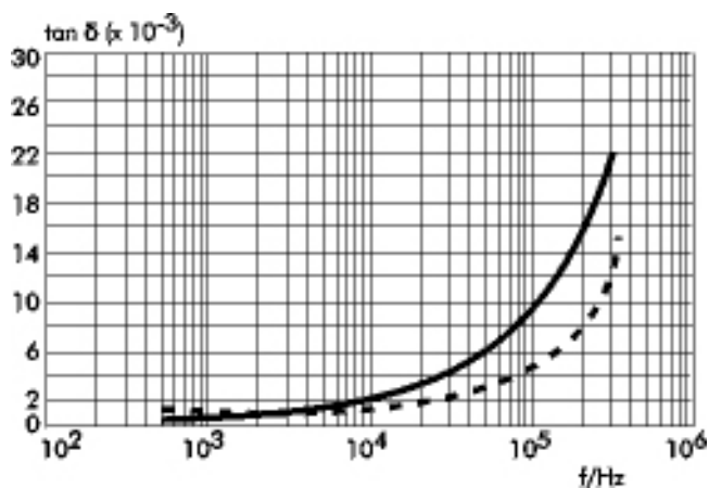
Dissipation factor change with frequency (general guide)
