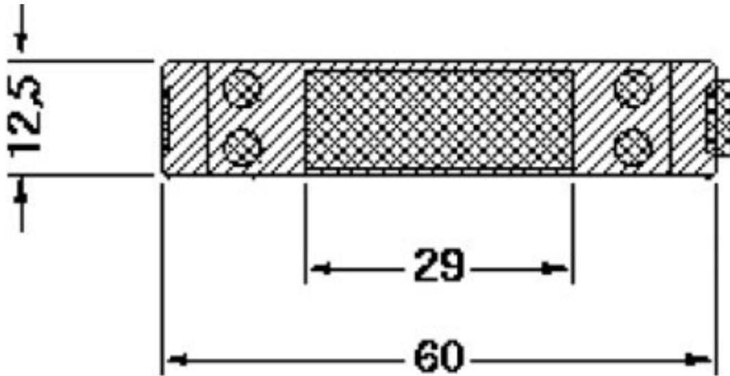
Dimensioned drawing
