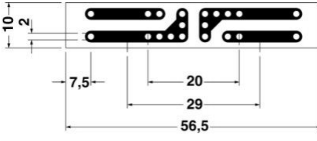
Dimensioned drawing
