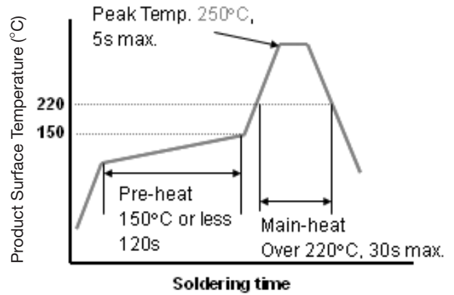
Reflow profile at 250°C.
