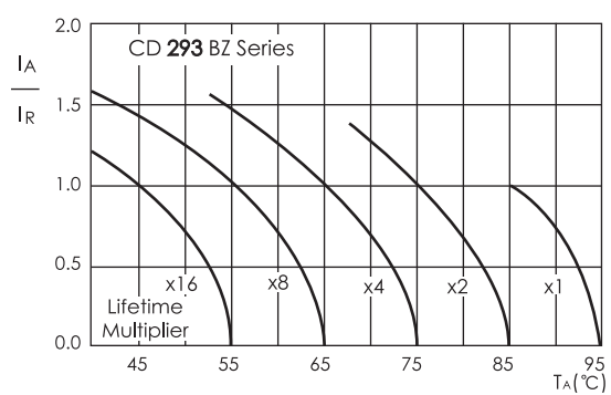
Lifetime Diagram U_r \geq 160V
