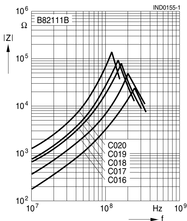
B82111B0000C016...C020
