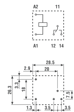
Copper side view Pin length 3.5 mm for PCB
