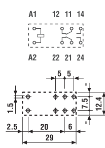
Copper side view Pin length 5.3 mm for PCB or sockets
