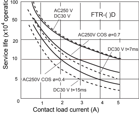
Life Curve
