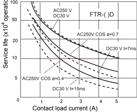
Life Curve
