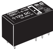
G5RL-1-E-HR
