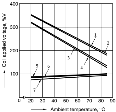
4-(1). Ambient temperature characteristics (1 Form A type) Tested sample: JQ1a-24V-F Contact carrying current: 3 A, 5 A
