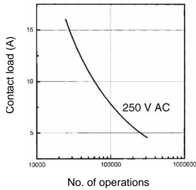
2. Life curve
