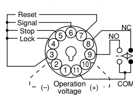
Relay output type
