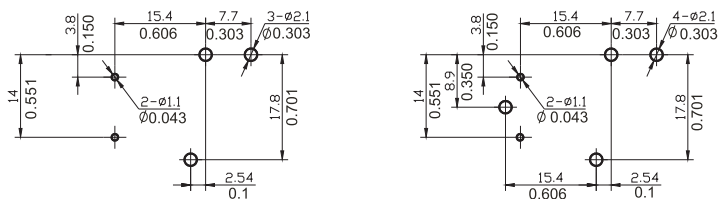
Mounting (Bottom view)
