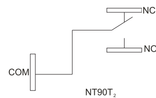
Wiring diagram(Top view)
