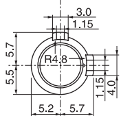
Pyro-Element
