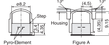
Pyro-Element
