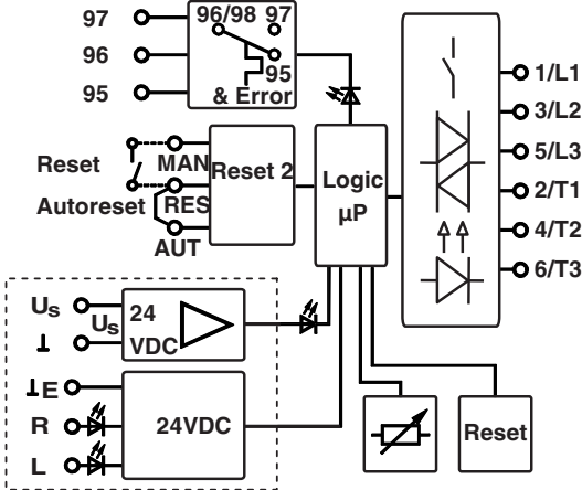
Figure 4 Block diagram
