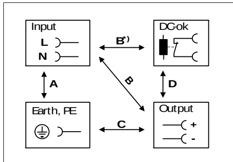
Fig. 18-1 Dielectric strength
