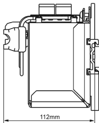
Fig. 2 Side view
