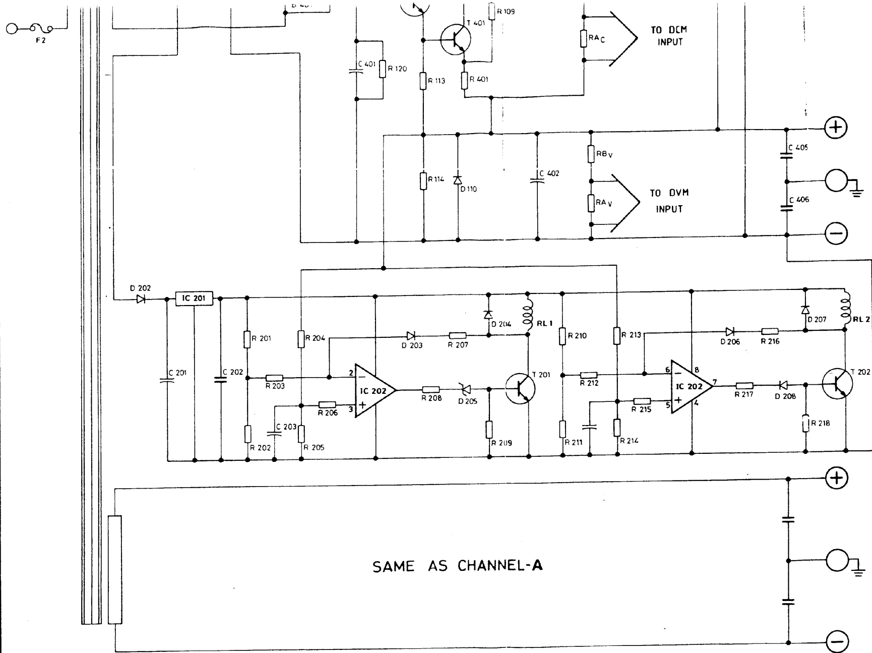
SCHEMATIC CIRCUIT DIAGRAM OF MODEL PS 2403
