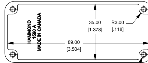
Top View Looking Inside Box
