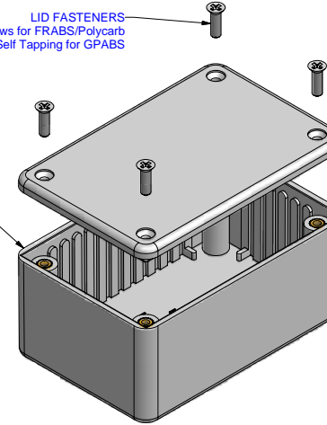
EXPLODED VIEW OF ASSEMBLY
