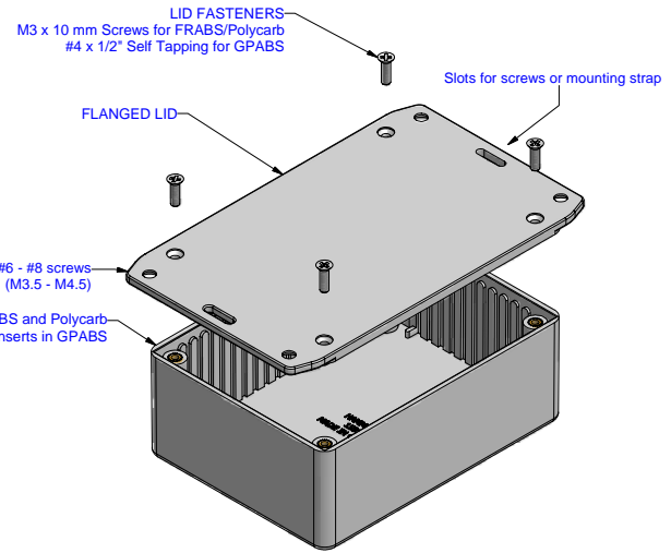
EXPLODED VIEW OF ASSEMBLY
