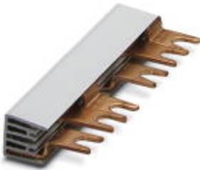
Wiring bridge for modules with connecting pitch 17.5 mm, 3-phase, 6-pos.
