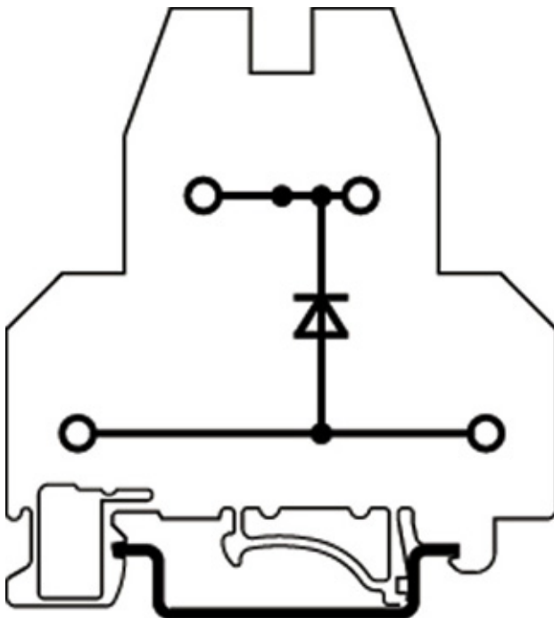
Circuit diagram
