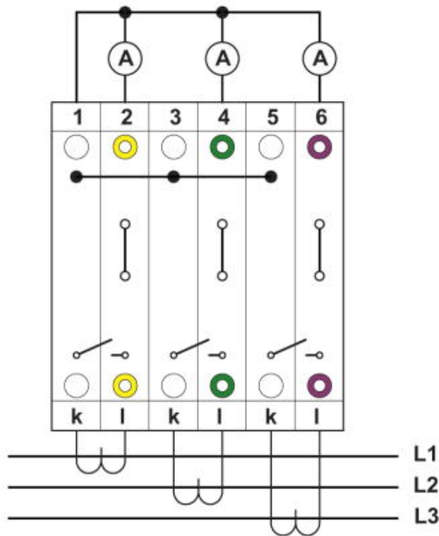
Connection diagram
