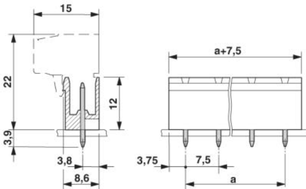
Dimensioned drawing
