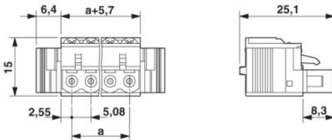
Dimensioned drawing
