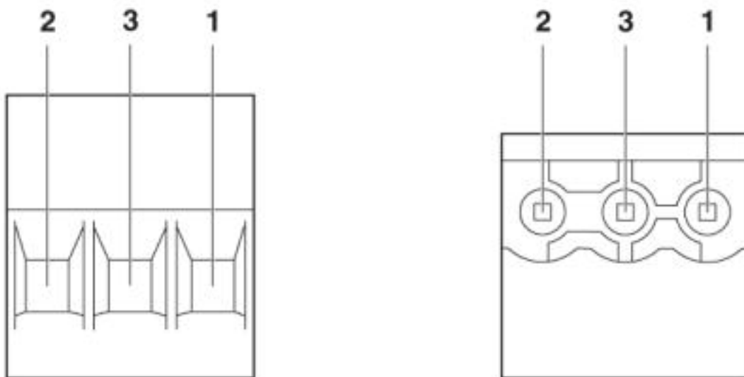
Pin assignment left
