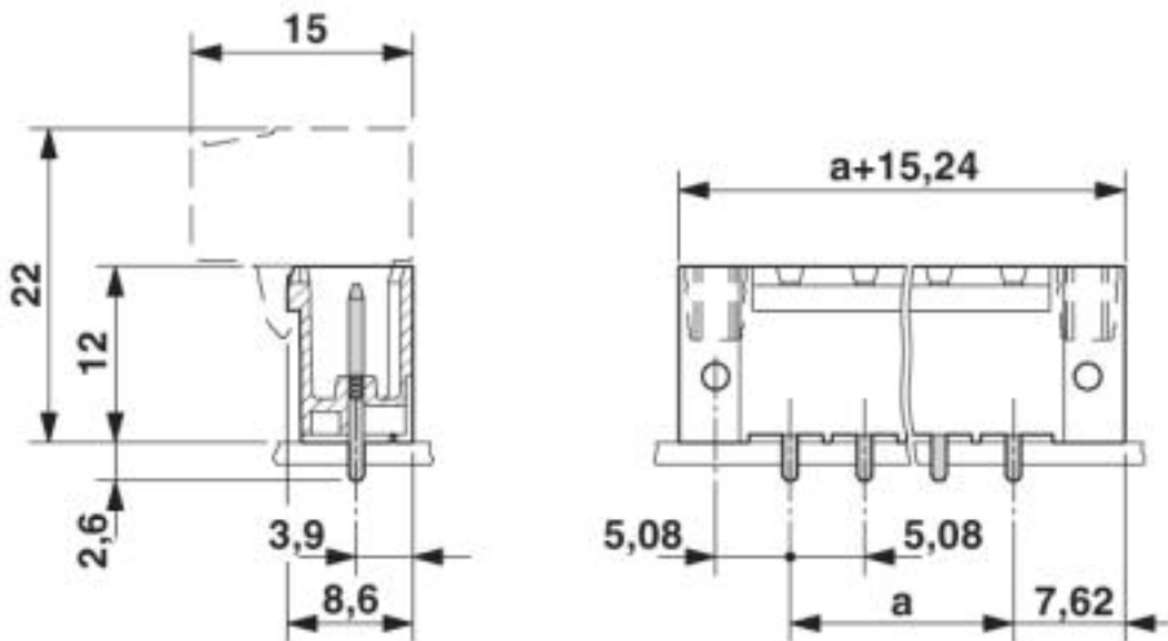
Dimensioned drawing
