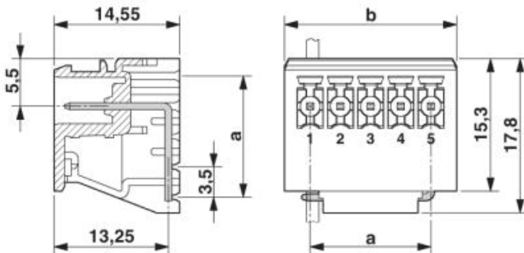
Dimensioned drawing
