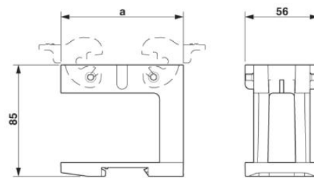
Dimensional drawing, a = 120 mm
