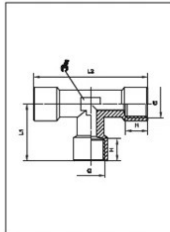
T-Stück Female Tee
