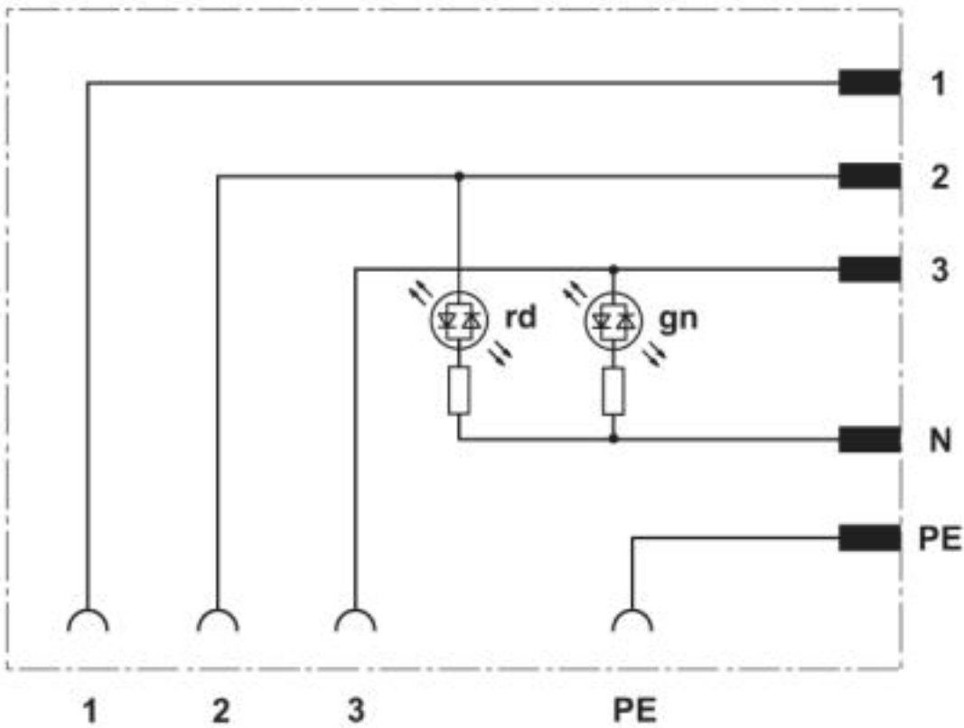
Circuit diagram
