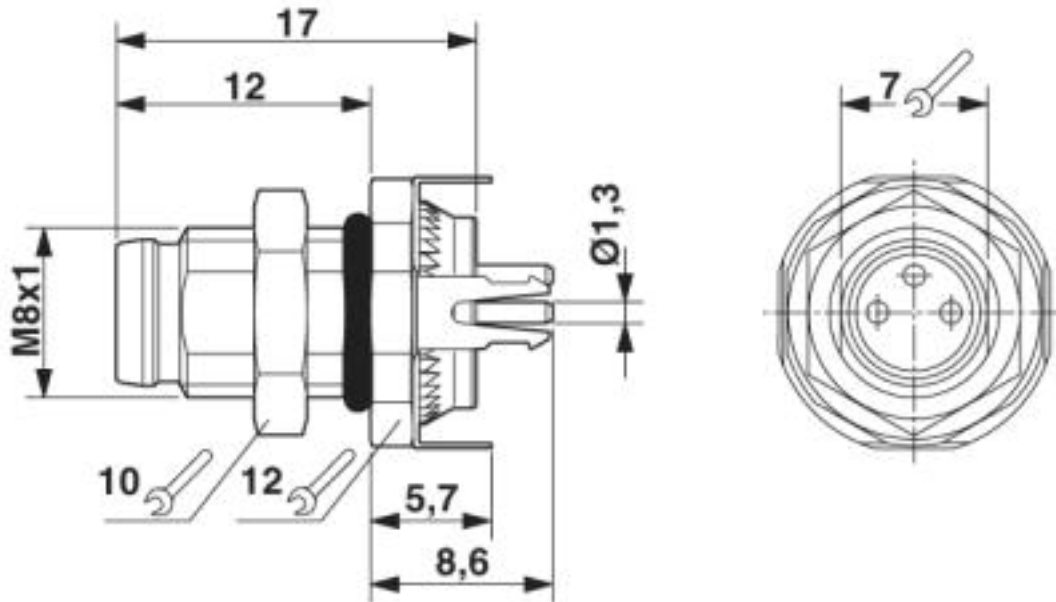
M8 flush-type plug, front mounting
