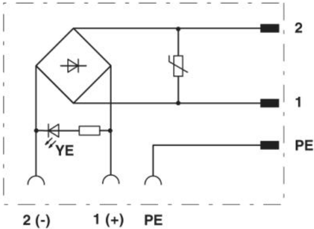
Circuit diagram
