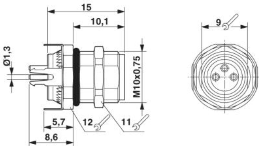
M8 flush-type socket
