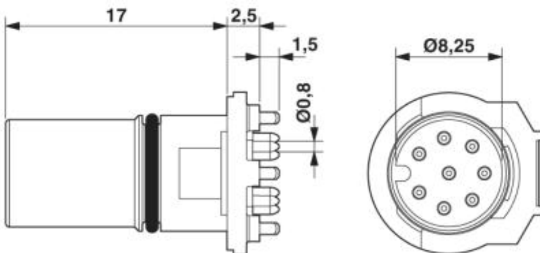
Dimensioned drawing
