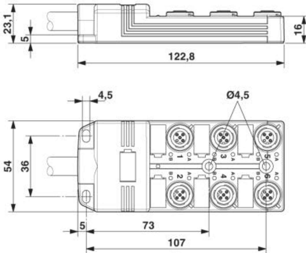
Dimensioned drawing
